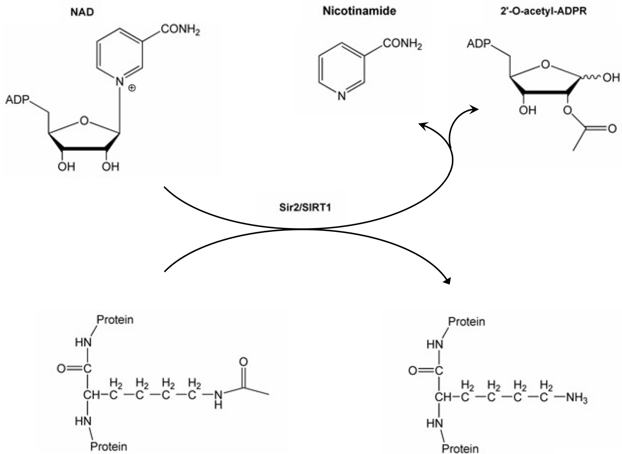
Figure 1. The NAD + -dependent SIRT1 deacetylase reaction
